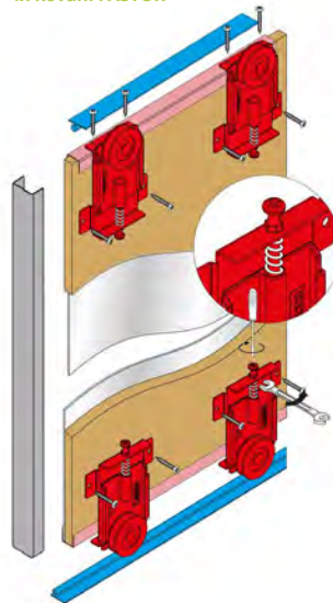
FASTOR FLAT (typ GAMA)
